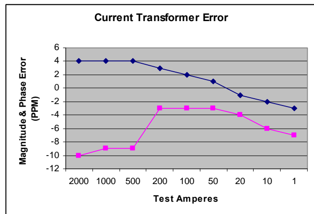
Error in the CT < 10 ppm ■ Phase ♦ Magnitude
